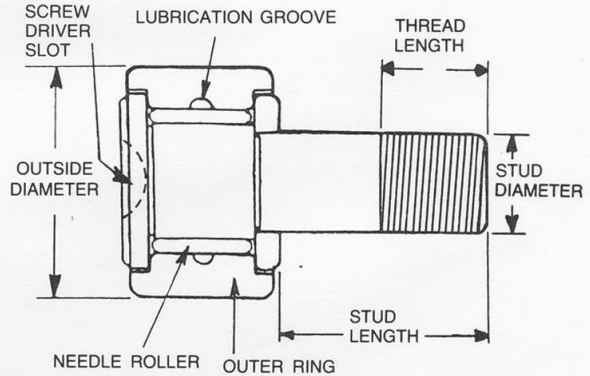
CAM FOLLOWER
